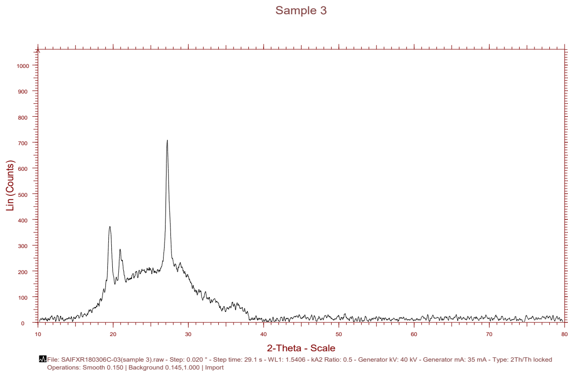
Figure.39 Zinc nanoparticle formation of (Sundari) dry fruit methanol extract under XRD imaging system.
